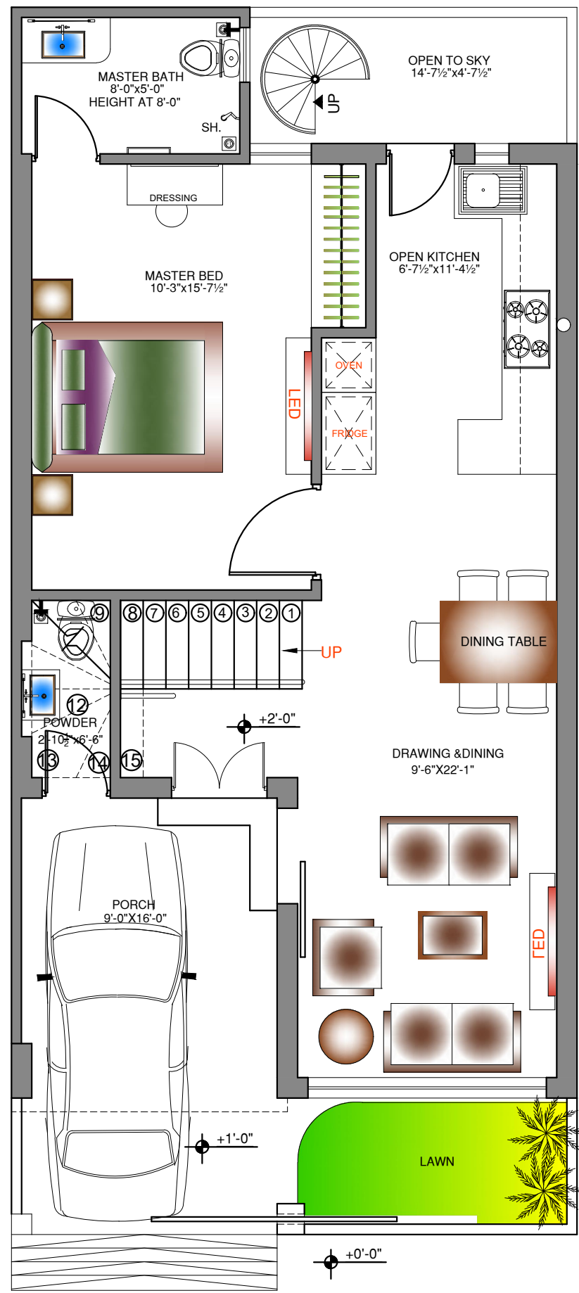
GROUND FLOOR COVERED AREA= 775 SQ.FT
