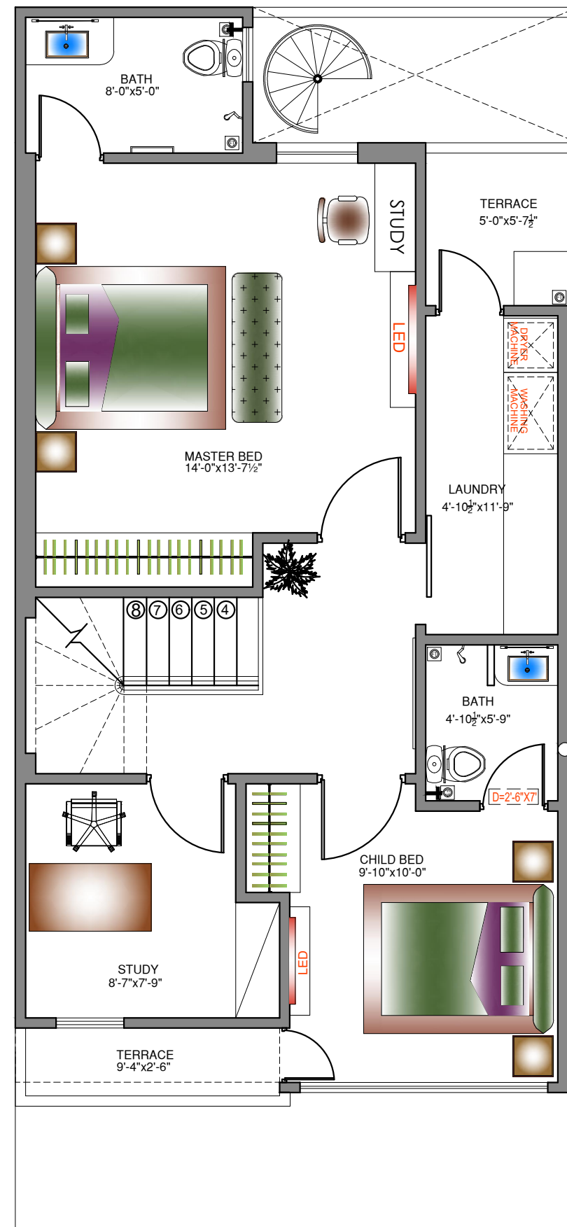
FIRST FLOOR COVERED AREA= 733 SQ.FT
