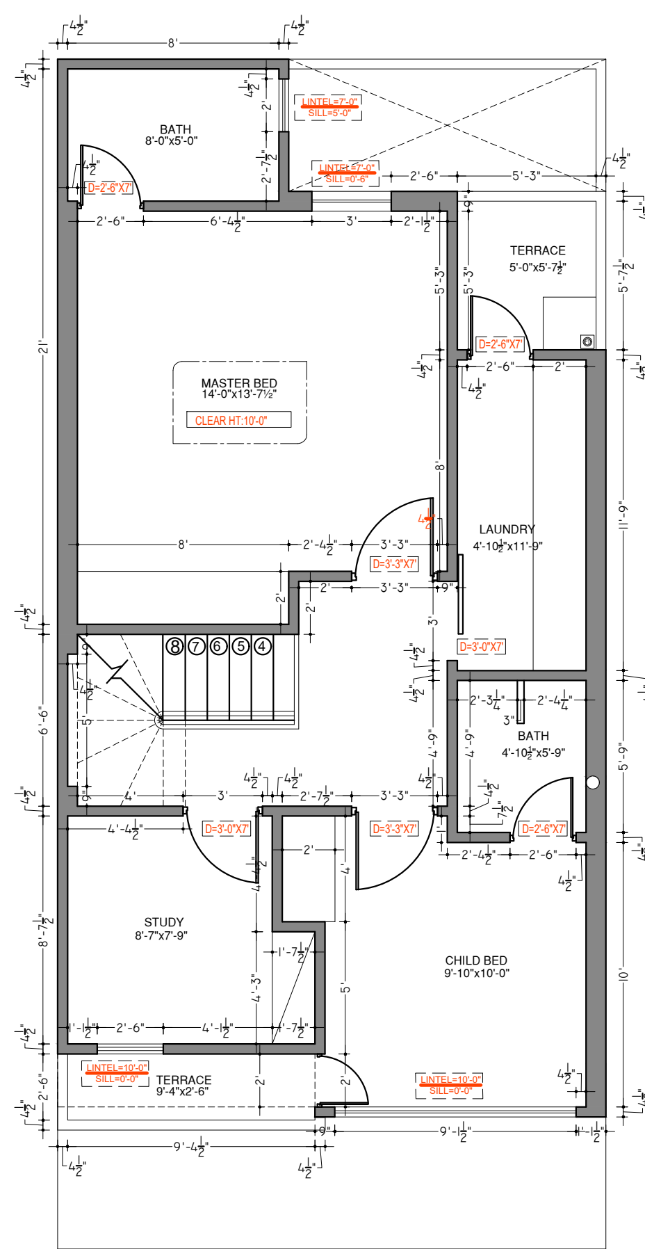
FIRST FLOOR COVERED AREA= 733 SQ.FT
