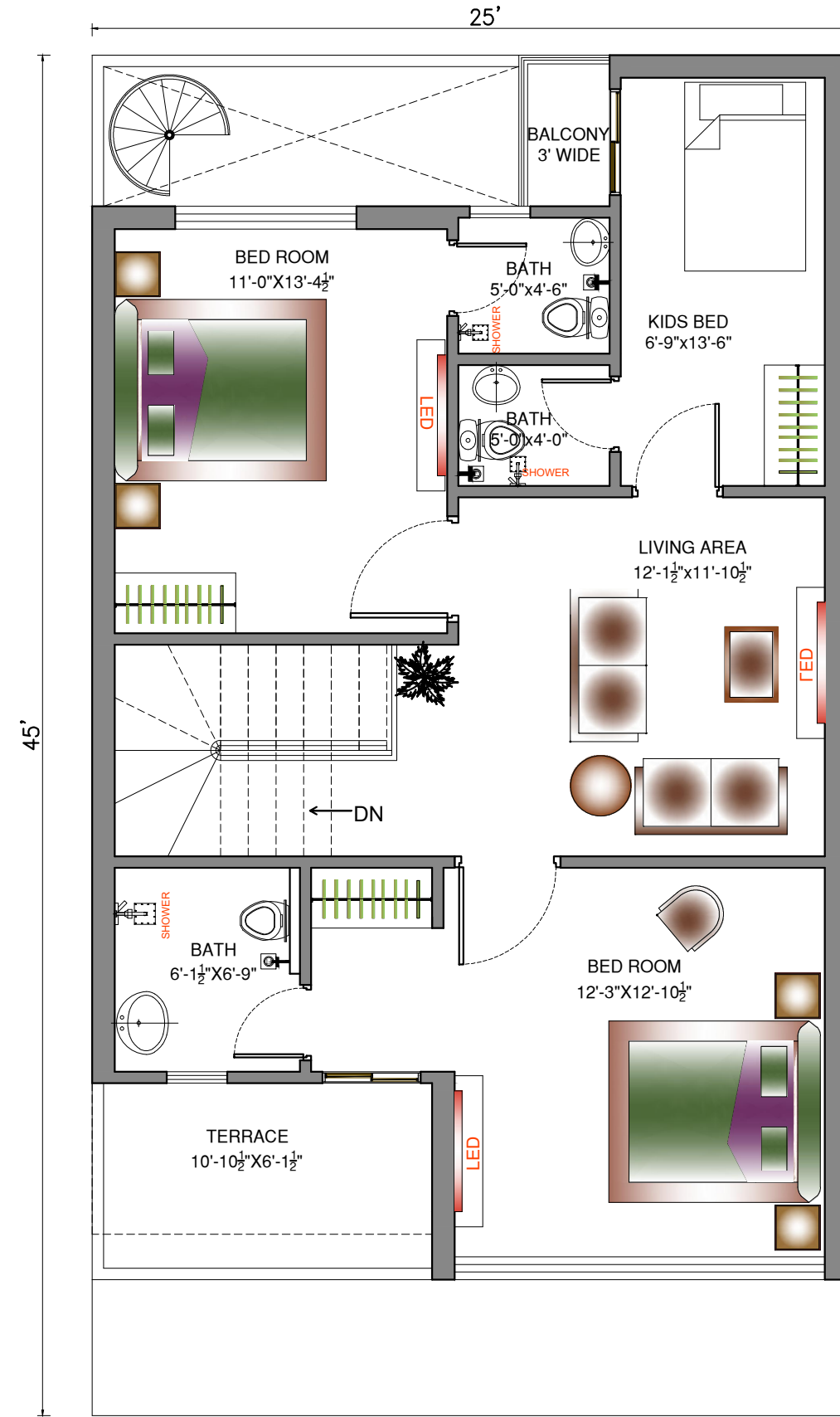
FIRST FLOOR COVERED AREA=910 SQ.FT
