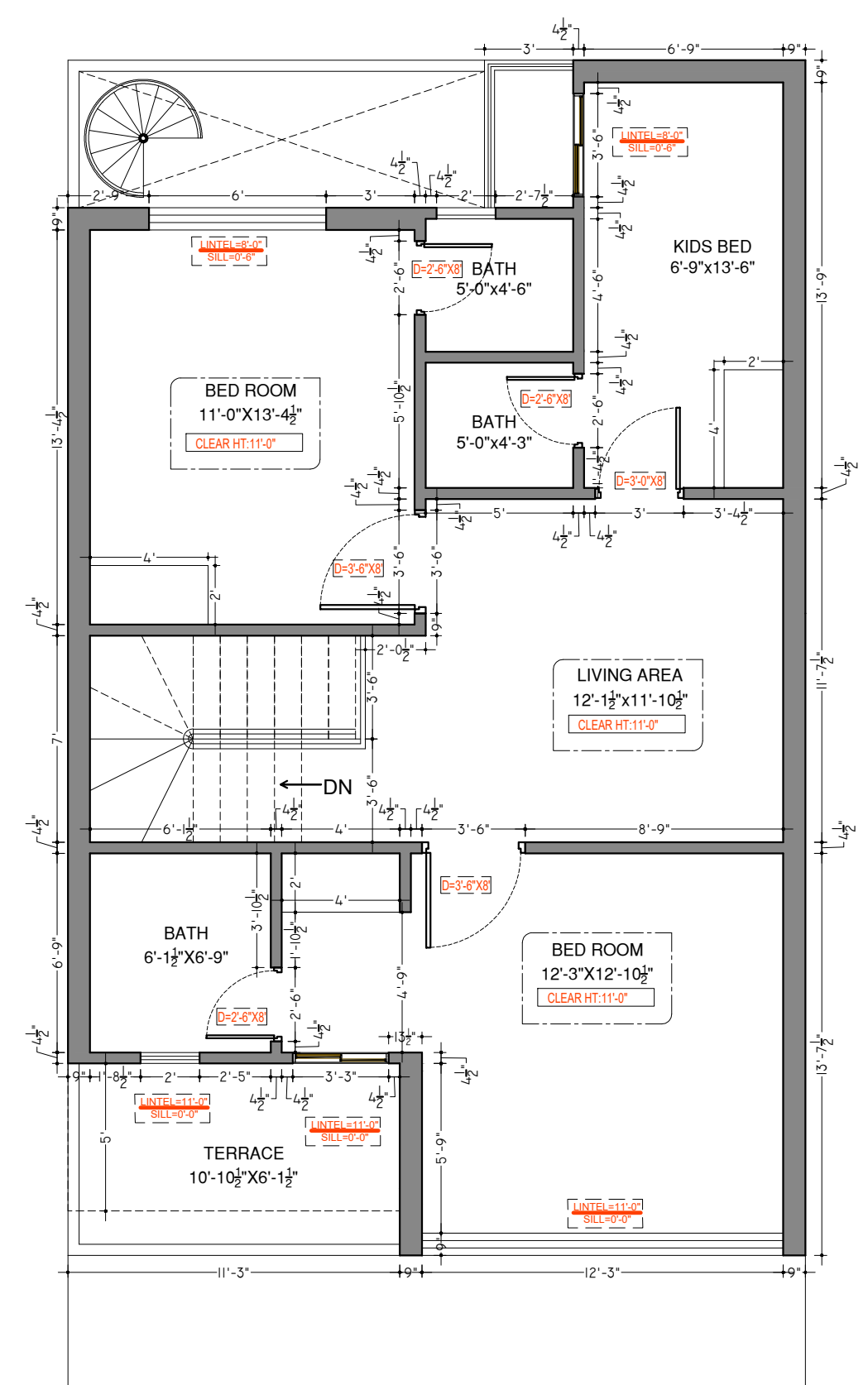
FIRST FLOOR COVERED AREA= 910 SQ.FT
