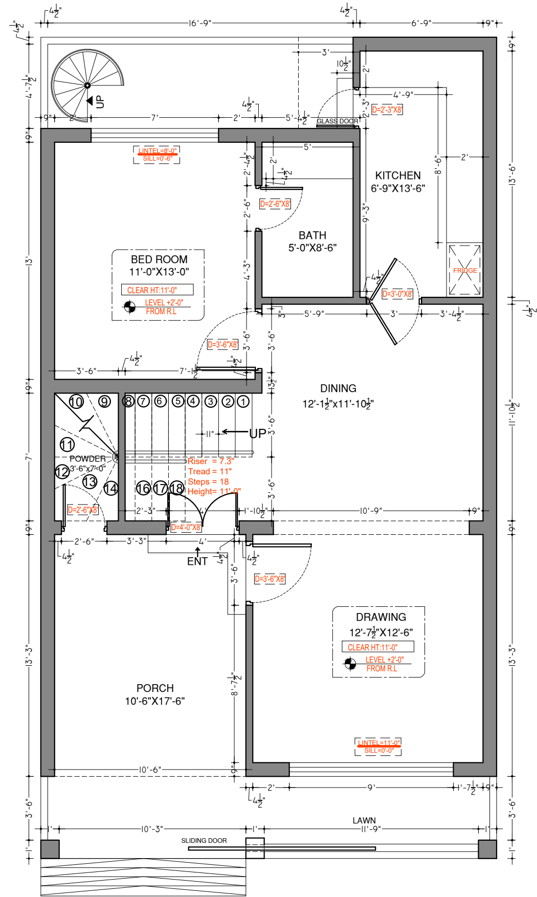
GROUND FLOOR COVERED AREA= 937 SQ.FT
