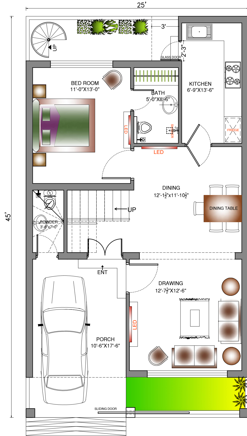
GROUND FLOOR COVERED AREA= 937 SQ.FT
